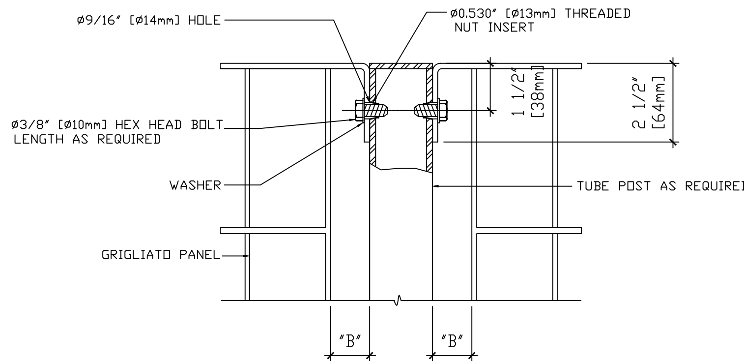
2 AI PANEL & POST ATTACHMENT DETAIL NOT TO SCALE
